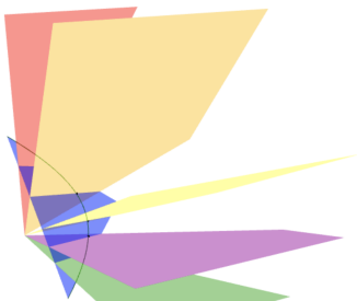
Log-normal spaces
