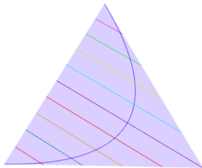
Log-normal polytopes
